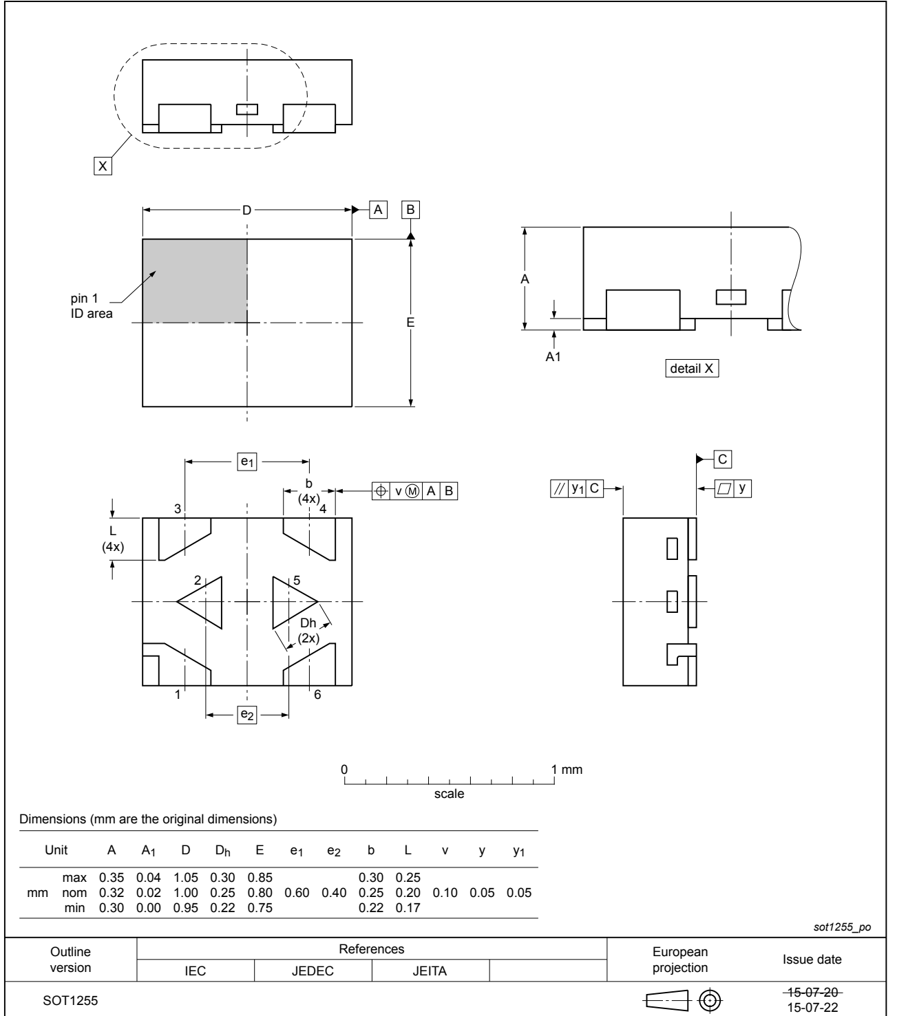
Fig. 1. Package outline X2SON6 (SOT1255)
